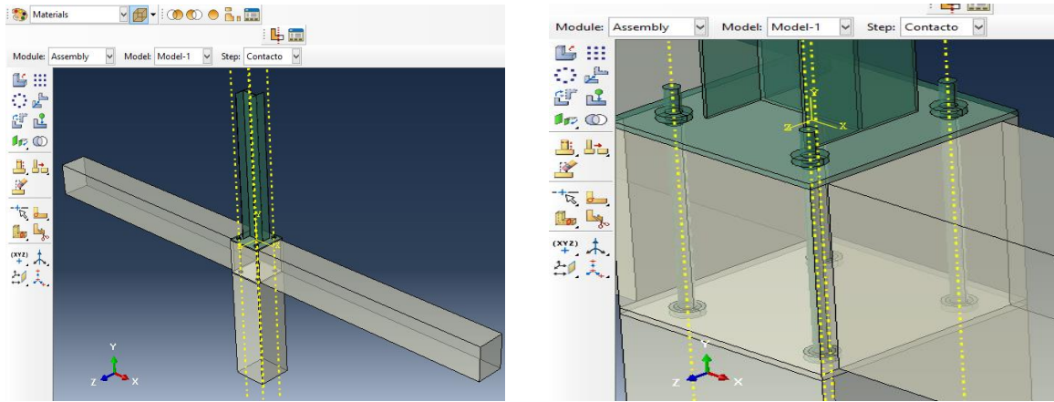
Figure 77. Distribution of materials in the model (Steel in green, concrete in beige). Source: [4]
