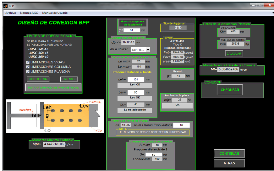
Figura 10. Interfaz principal BFP
