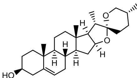
Diosgenina ( 19 )
