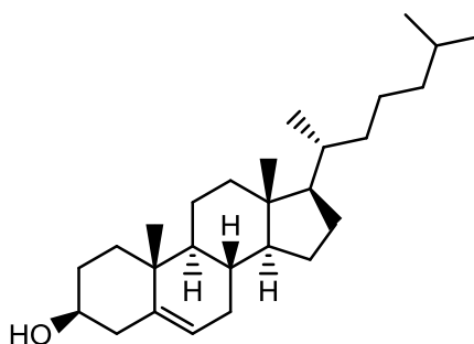
Colesterol (25)
